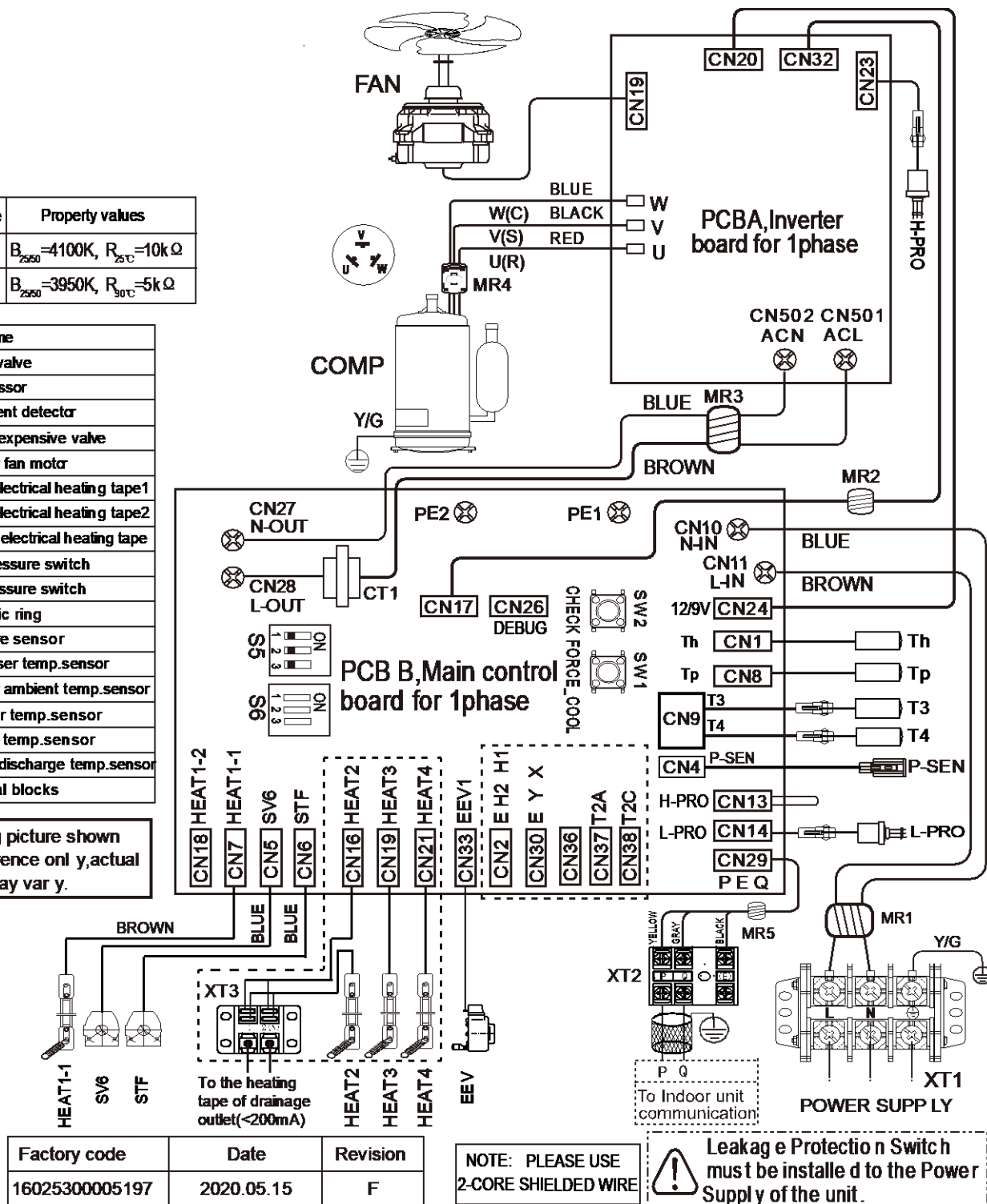
Figure 2-4.1: ECOSPAR-S12(14,16)kW-1N wiring diagram
