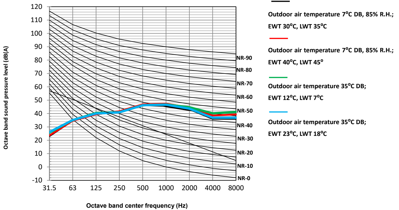
Figure 2-8.8: ECOSPAR-S12kW-3N octave band levels
