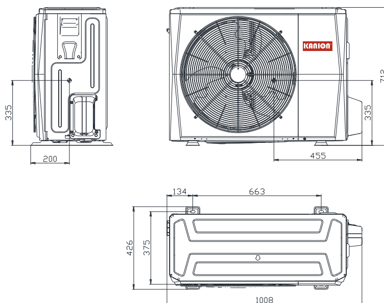
Figure 2-2.1: Dimensions and center of gravity (unit: mm)
