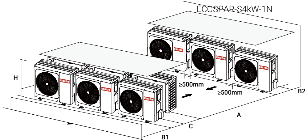
Figure 3-2.11: Multi-row installation
