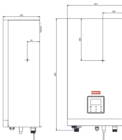
Figure 2-2.3: Dimensions and center of gravity (unit: mm)
