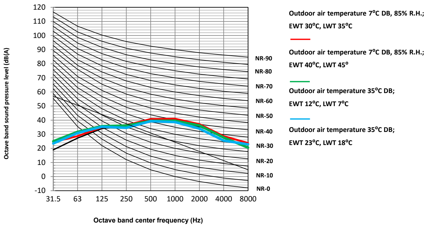
Figure 2-8.2: ECOSPAR-S4kW-1N octave band levels
