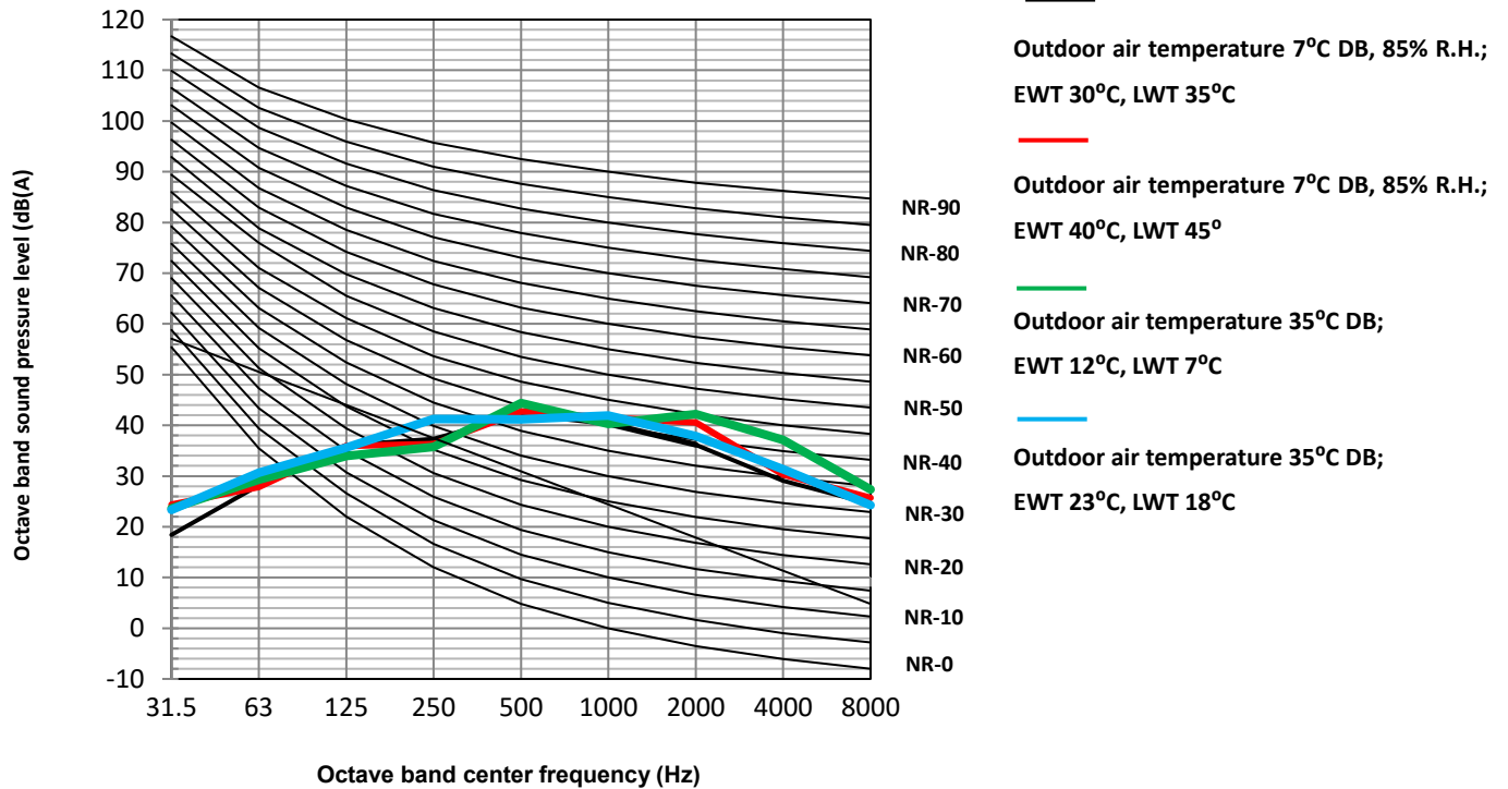
Figure 2-8.3: ECOSPAR-S6kW-1N octave band levels
