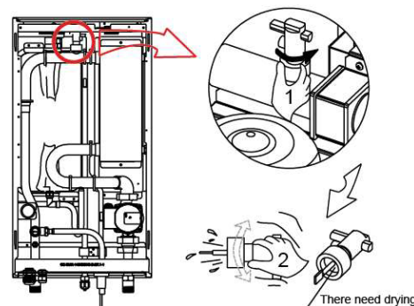
Figure 3-4.2: Water flow switch
