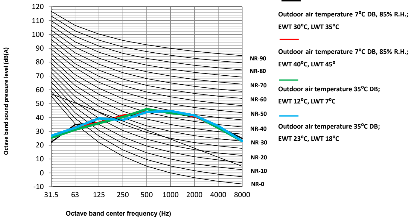
Figure 2-8.4: ECOSPAR-S8kW-1N octave band levels
