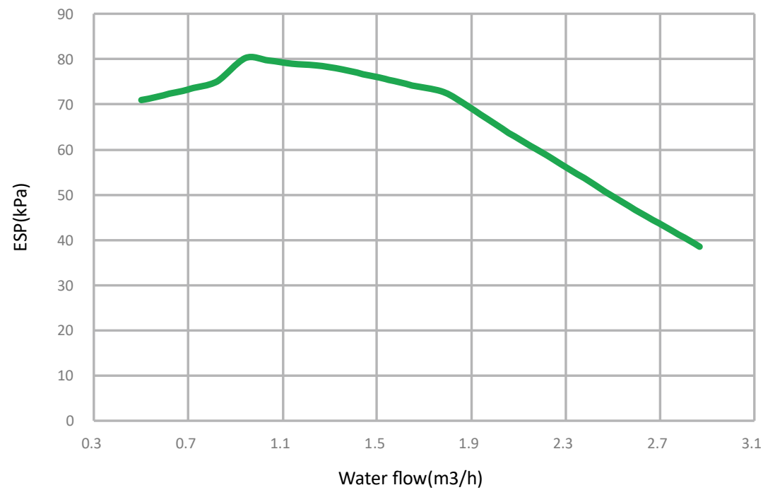
Figure 2-7.2: ECOSPAR-12kW~16kW hydronic performance
