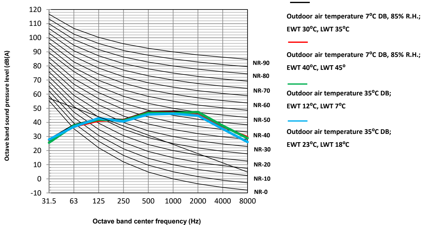
Figure 2-8.7: ECOSPAR-S14kW-1N octave band levels
