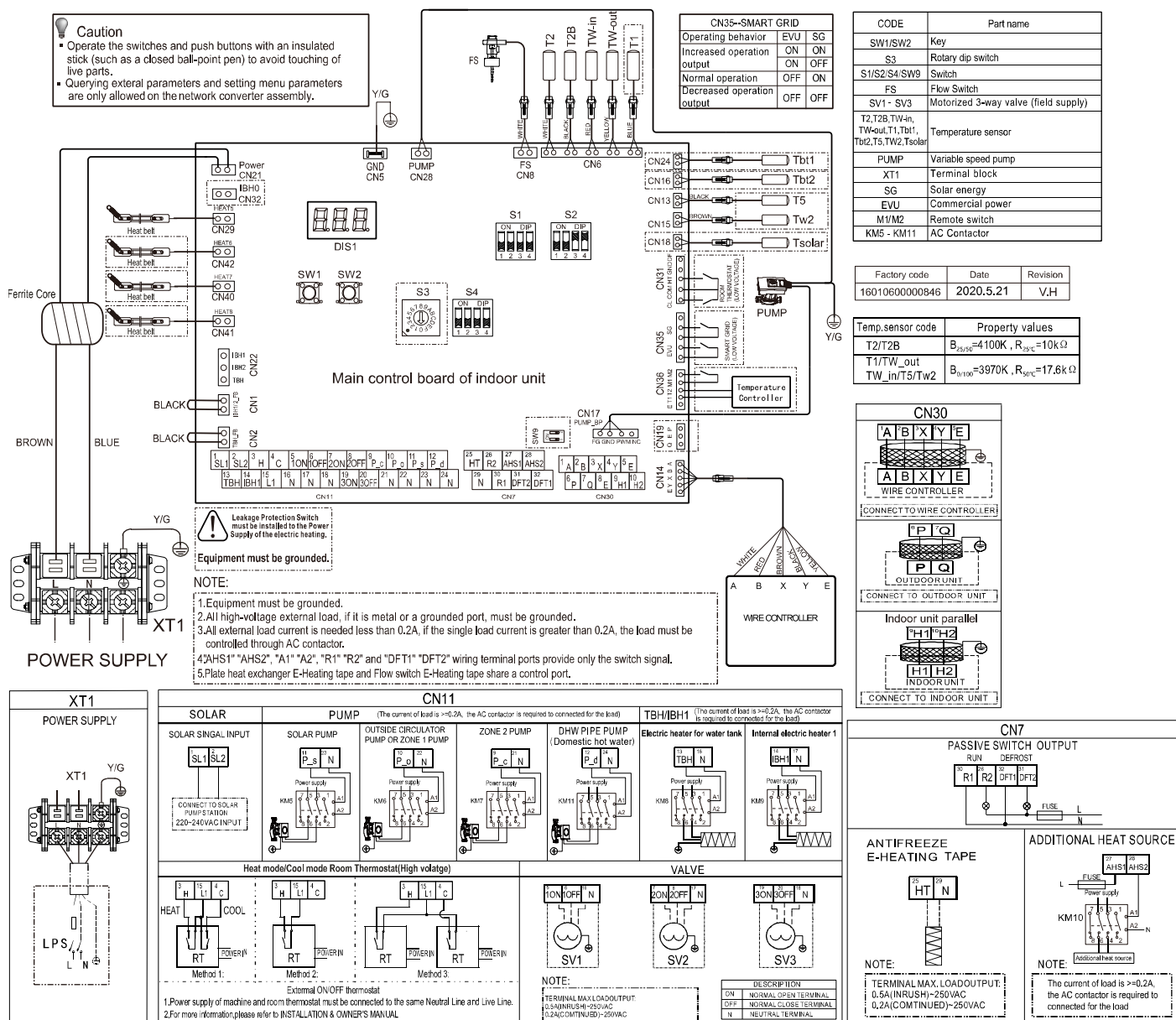
Figure 2-4.2 ECOSPAR-4kW~6kW(8kW~10kW, 12kW~16kW)Indoor wiring diagram
