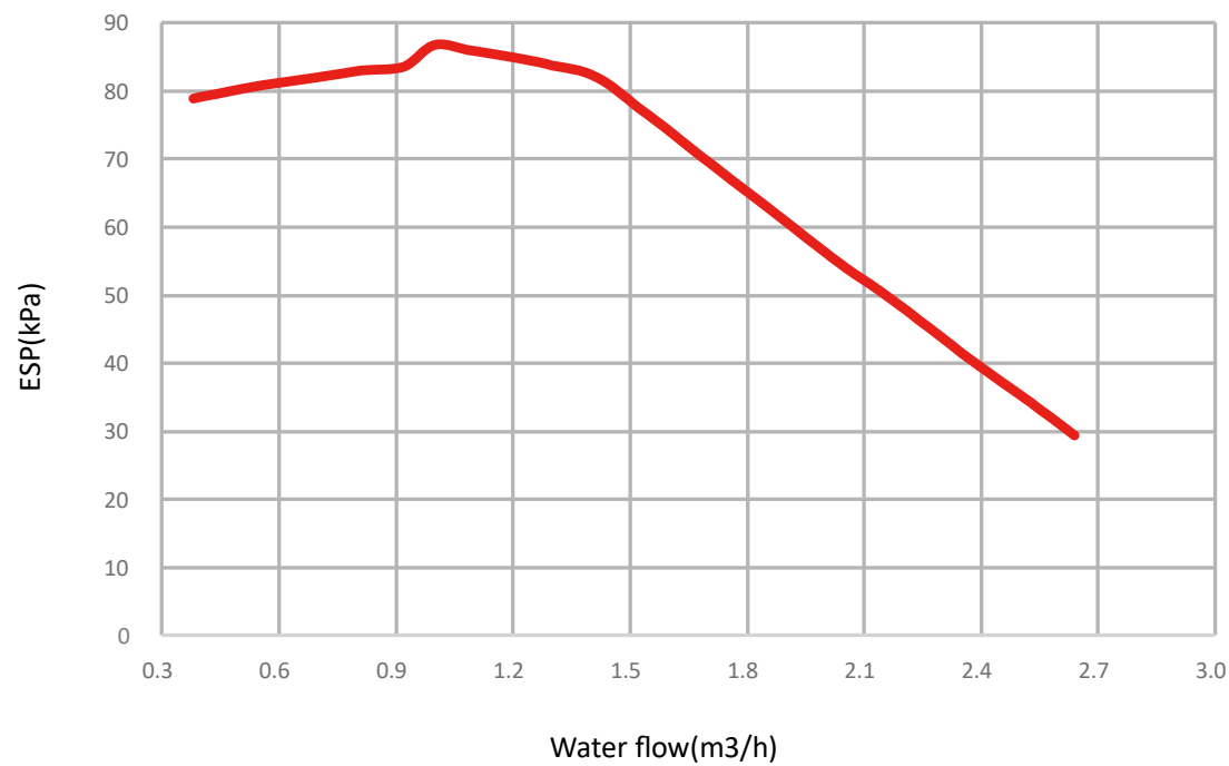
Figure 2-7.2: ECOSPAR-12kW~16kW hydronic performance
