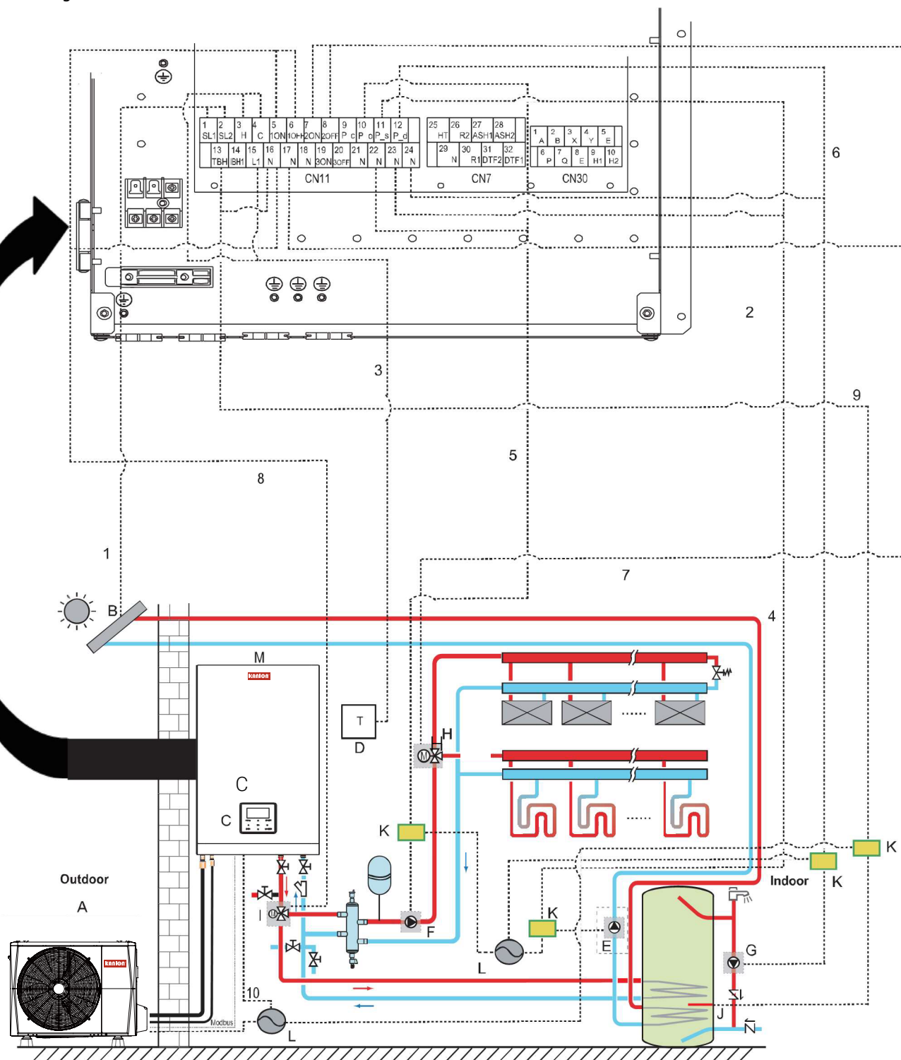
Figure 3-5.1: Wiring overview
