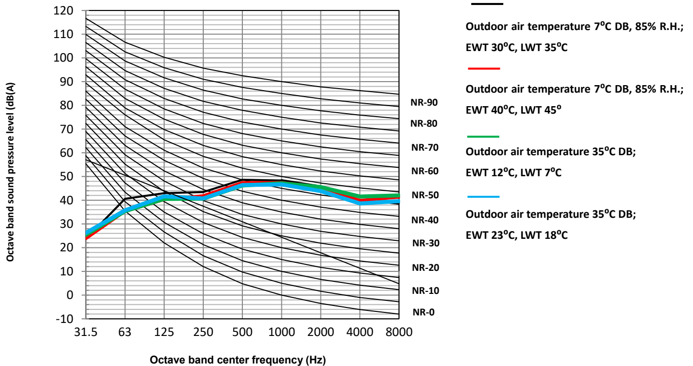
Figure 2-8.9: ECOSPAR-S14kW-3N octave band levels
