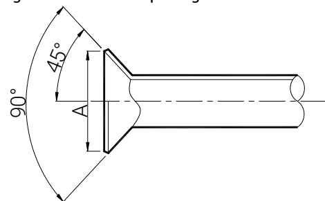
Figure 33.3: Flared opening
