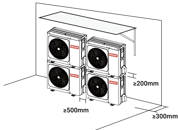
Figure 3-2.9: Installation with obstacles behind the unit
