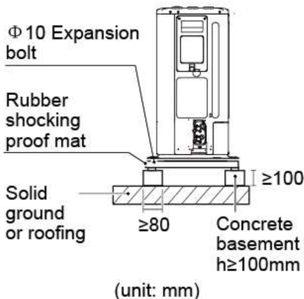
Figure 3-2.3: Outdoor unit fixing
