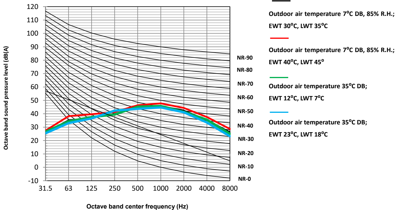
Figure 2-8.5: ECOSPAR-S10kW-1N octave band levels
