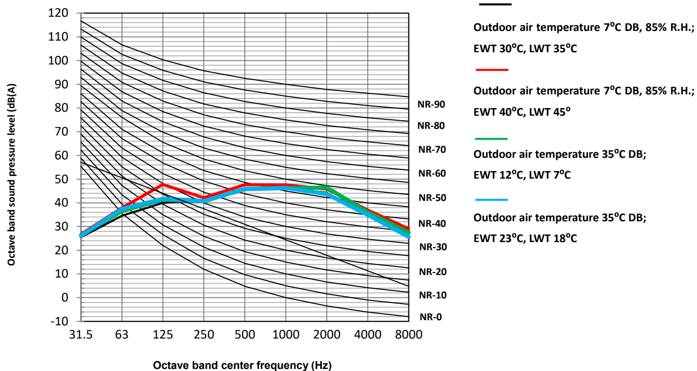
Figure 2-8.6: ECOSPAR-S12kW-1N octave band levels
