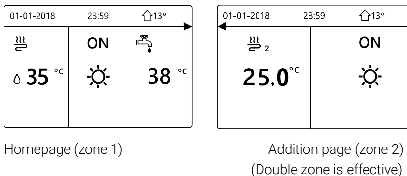
Figure 3-8.24: Set DOUBLE ZONE and ROOM TEMP. to YES; Set WATER FLOW TEMP. to YES or NON
