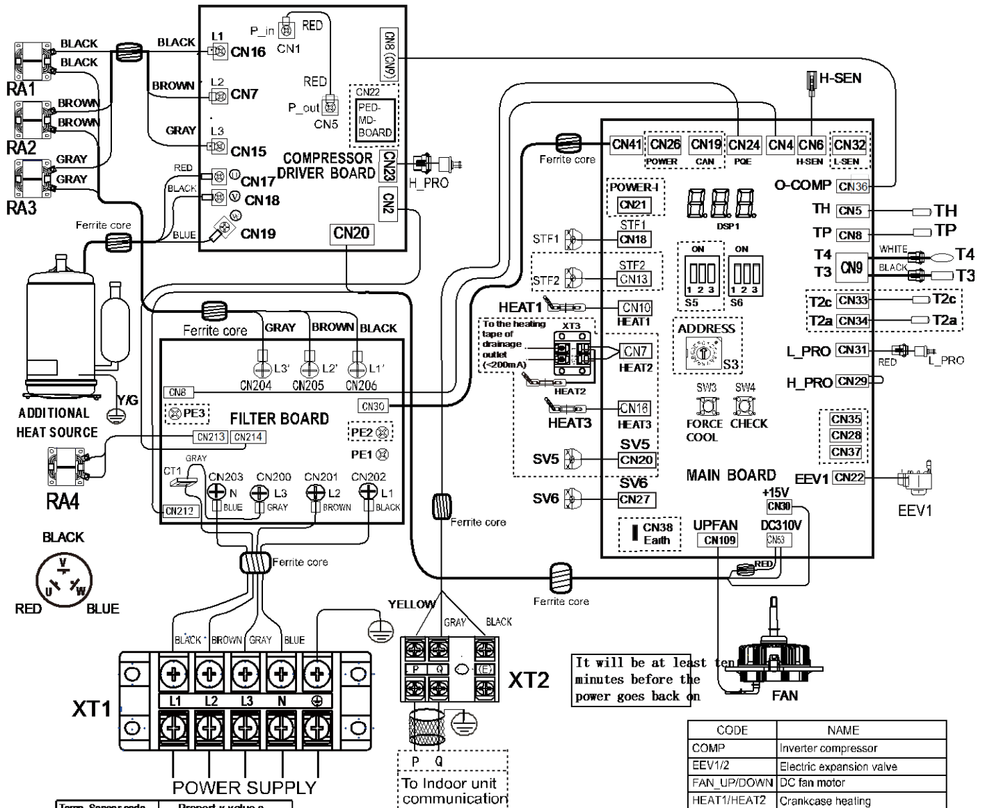
Figure 2-4.1: ECOSPAR-S12(14,16)kW-3N wiring diagram
