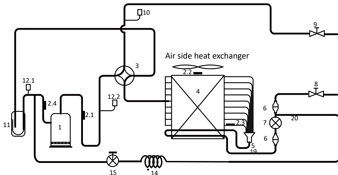
Figure 2-3.1: Outdoor unit piping diagram
