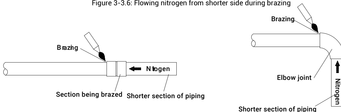
Figure 3-3.6: Flowing nitrogen from shorter side during brazing
