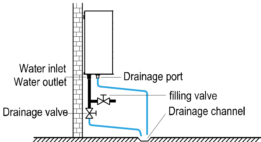
Figure 3-2.16: Drainage
