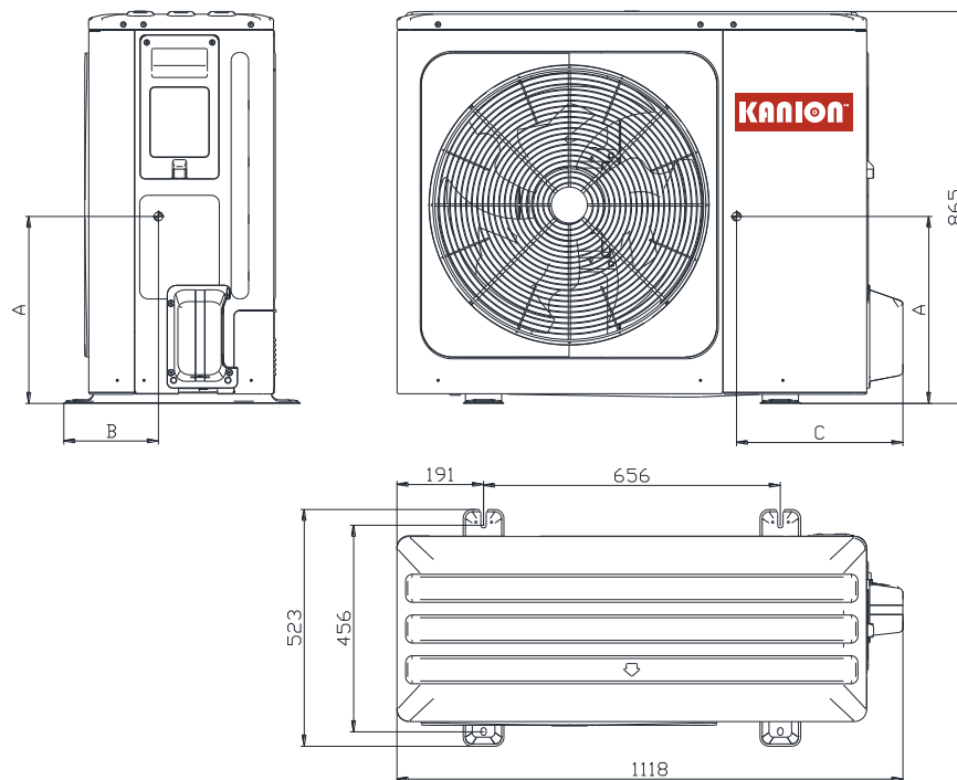
Figure 2-2.2: Dimensions and center of gravity (unit: mm)
