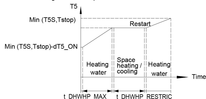
Figure 3-8.9: Operation DHW PRIORITY
